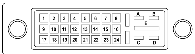
DVI-I CONNECTOR
